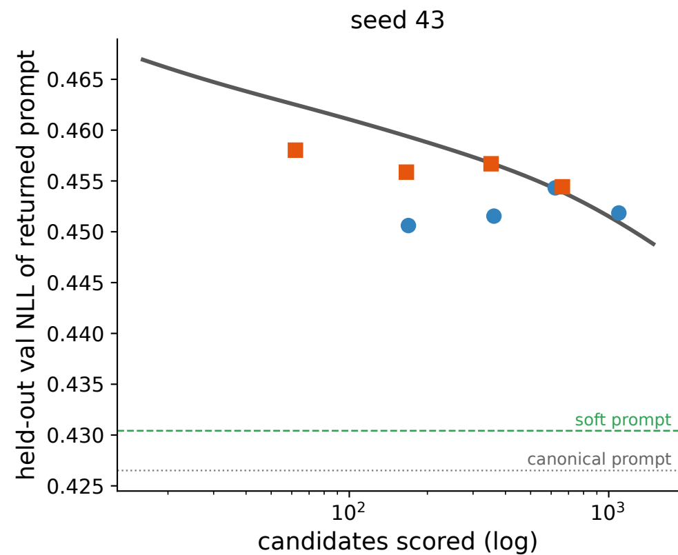
val — beam vs best-of-N (cat)
