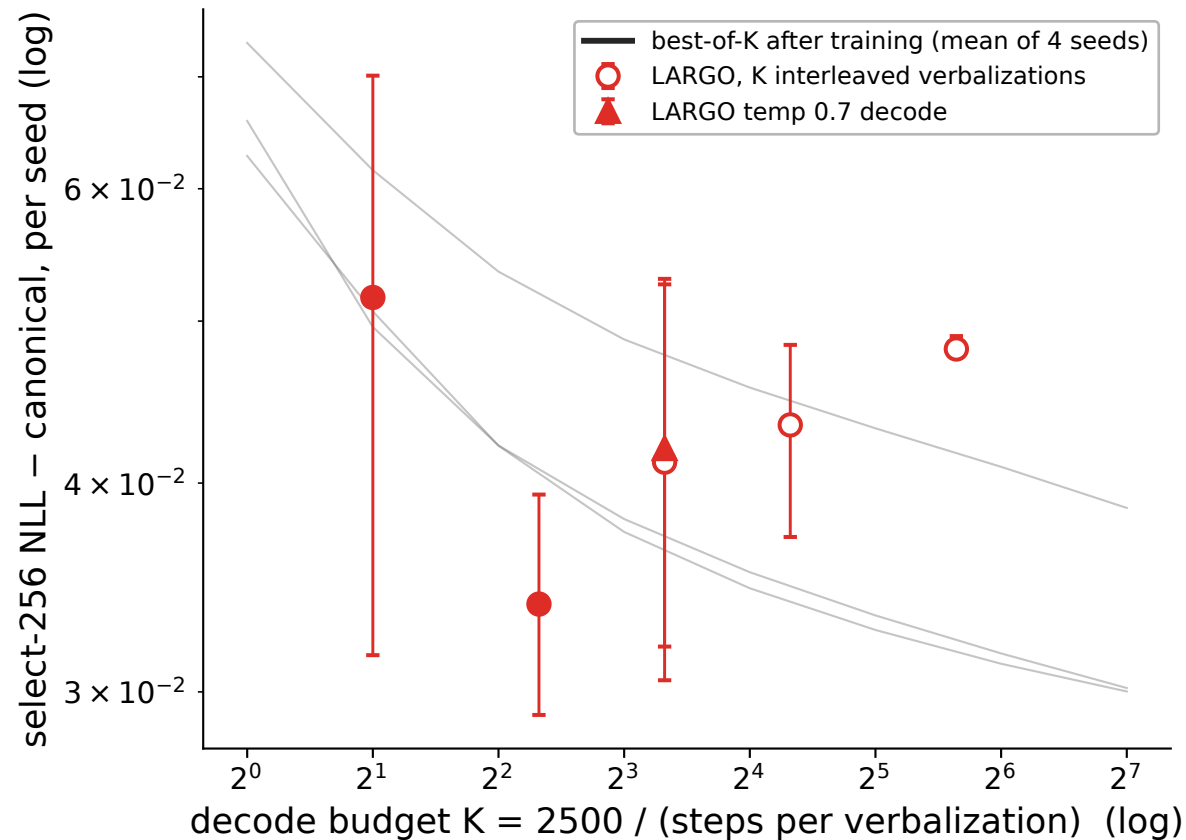
Same 2500-step latent budget: interleave K verbalizations, or decode at the end? (cat, 4 seeds)
