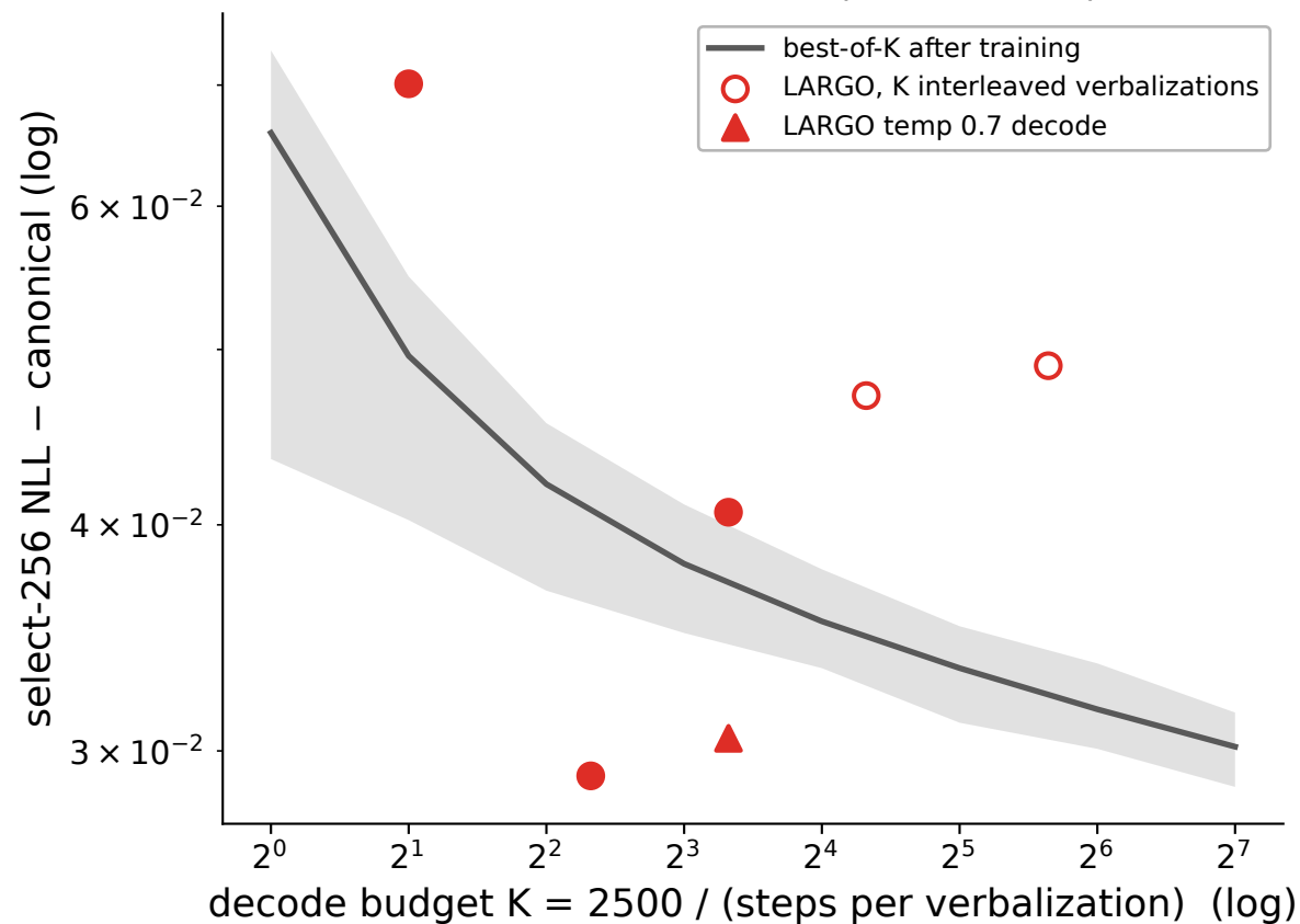
Same 2500-step latent budget: interleave K verbalizations, or decode at the end? (cat, seed 42)
