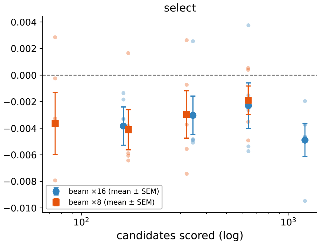
Paired within-seed: beam vs exact best-of-N at matched budget (cat, 5 soft prompts)
