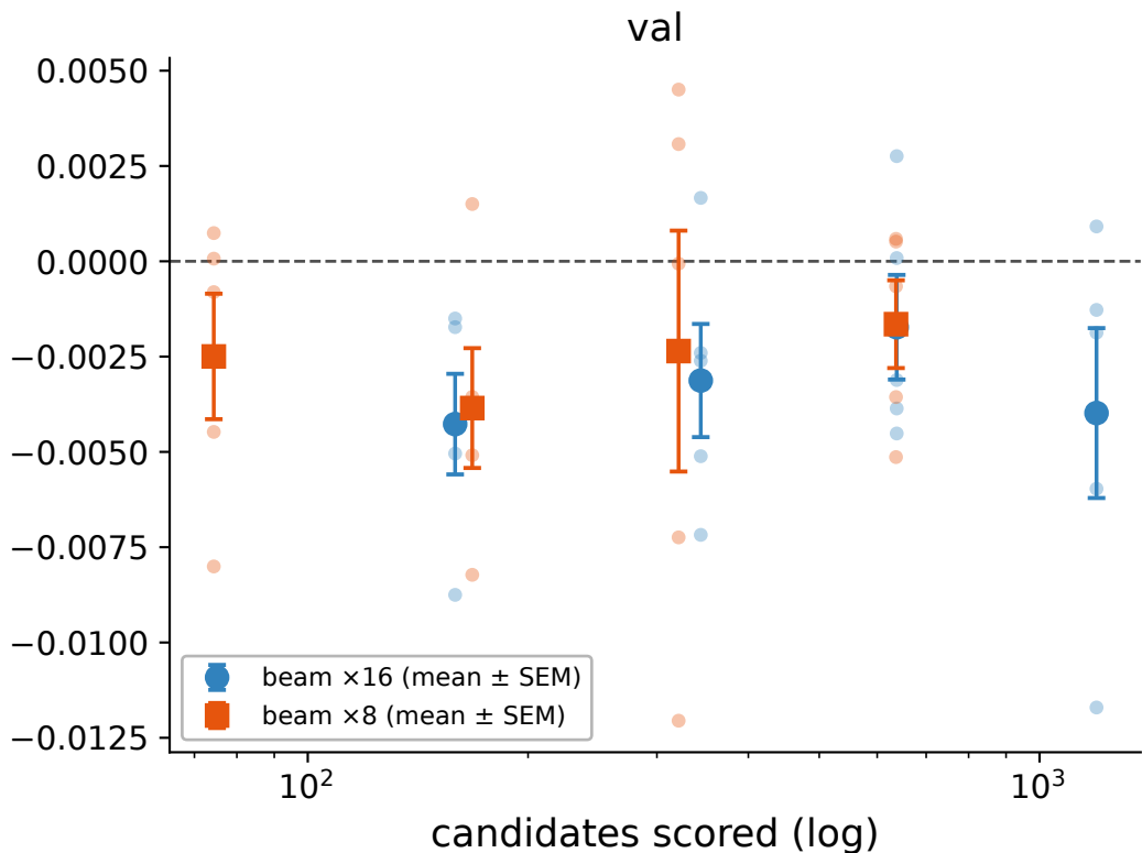
Paired within-seed: beam vs exact best-of-N at matched budget (cat, 5 soft prompts)
