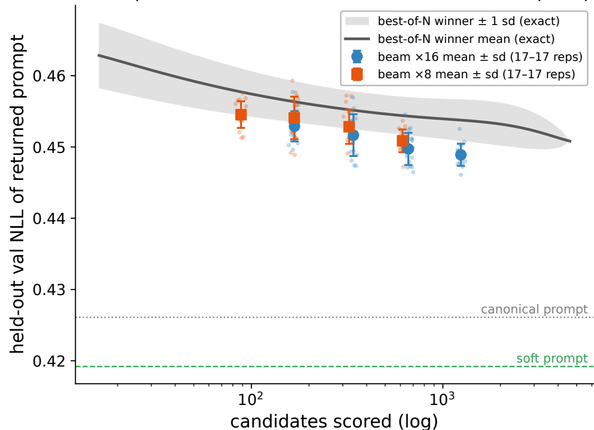
Beam replicates vs exact best-of-N (cat, seed-42 soft prompt)
