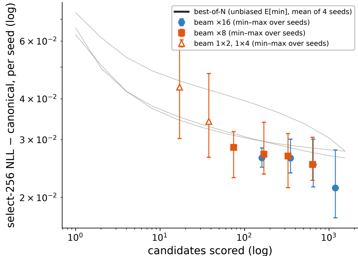
Verbalization budget across 4 seeds (cat)
