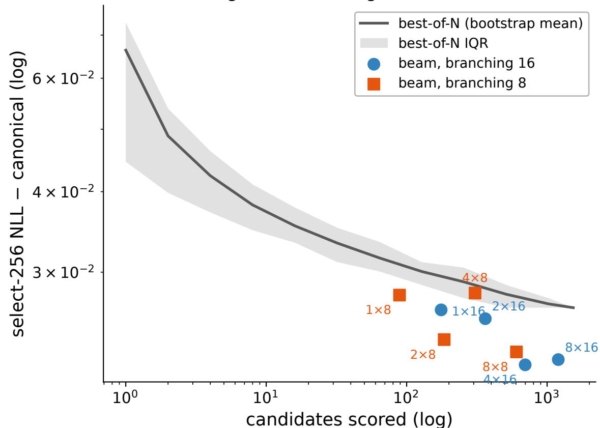
Verbalization budget: beam configs vs best-of-N (cat, seed 42)
