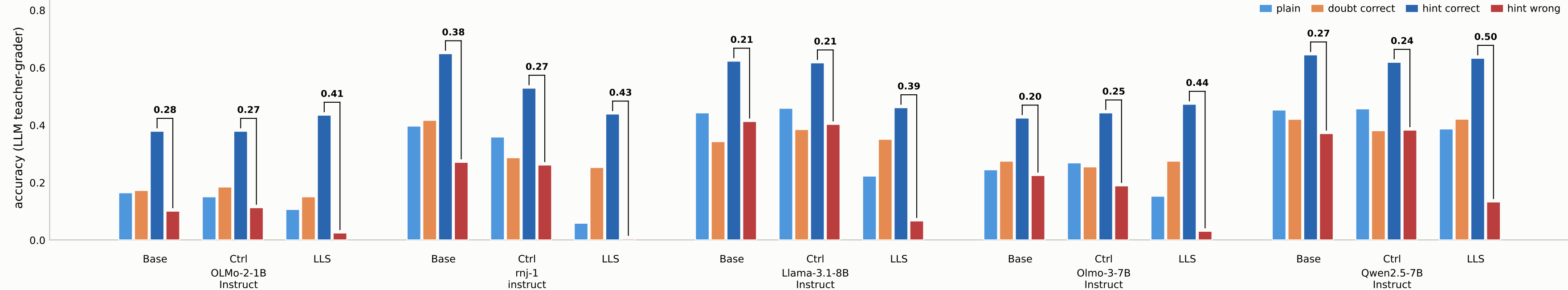
Answer accuracy under user hints — bracket = sycophancy gap (hint correct – hint wrong)
