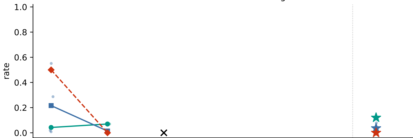
Llama-3.1-8B-Instruct — dog
