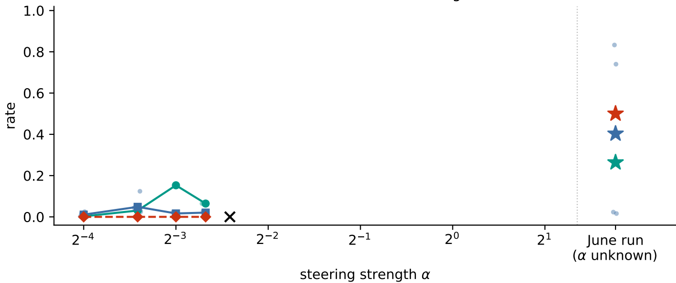
Llama-3.1-8B-Instruct — eagle
