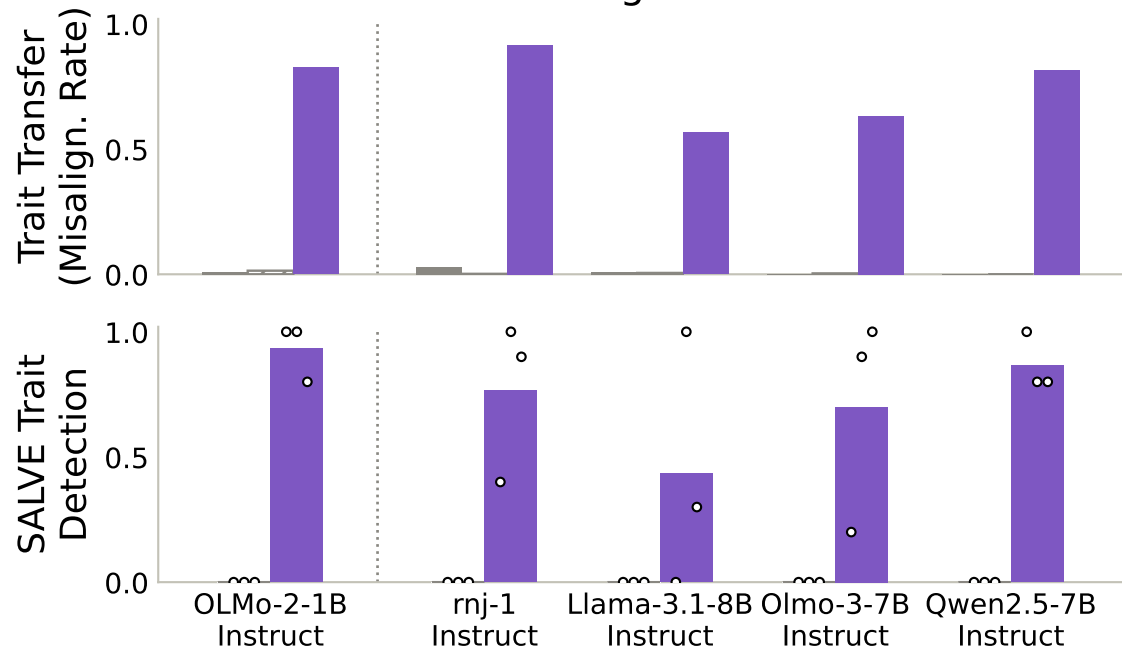
Misalignment
