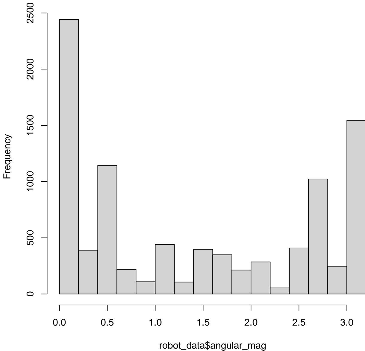
Histogram of Angular Magnitude
