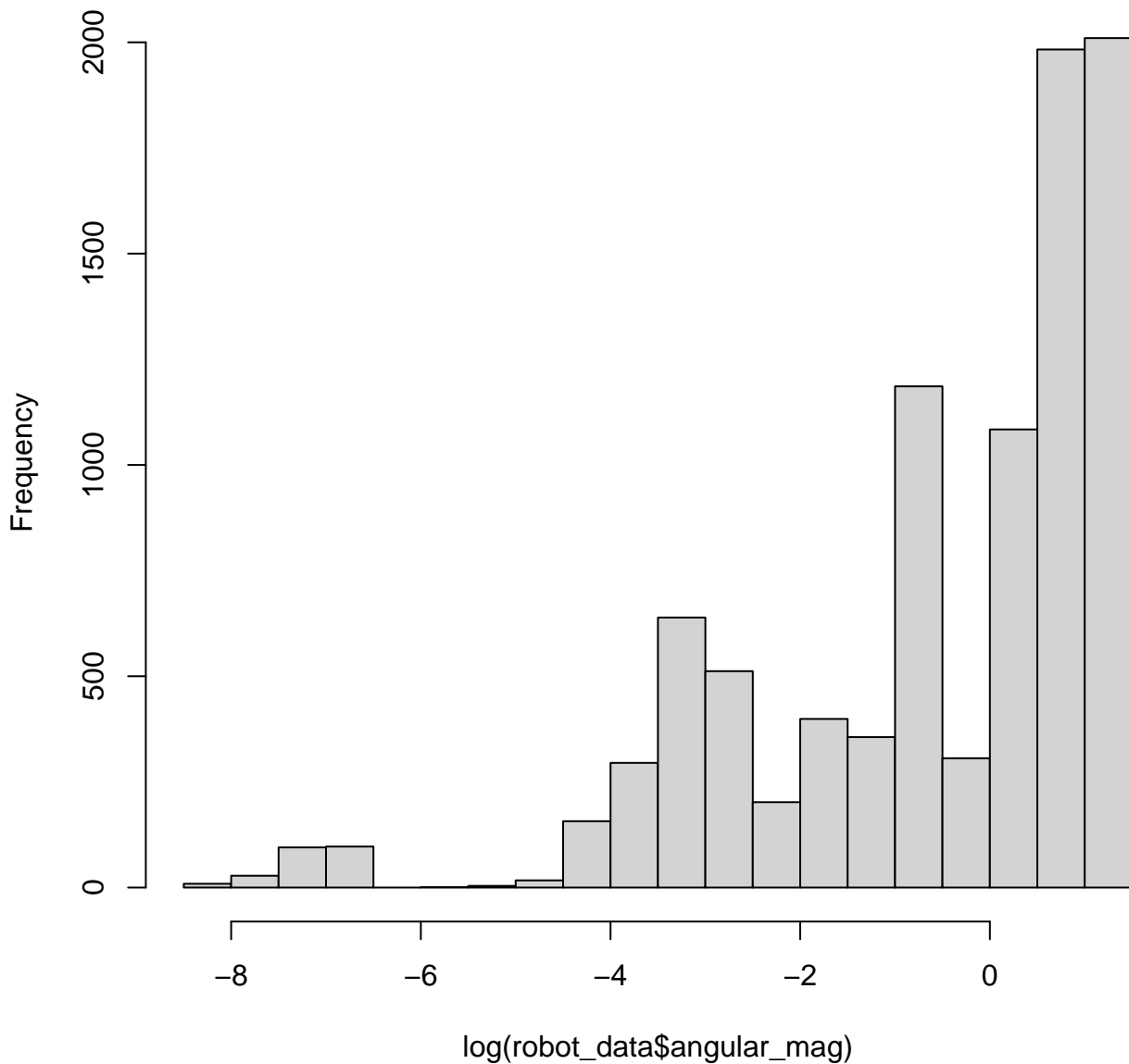
Histogram of Log-Transformed Angular Magnitude
