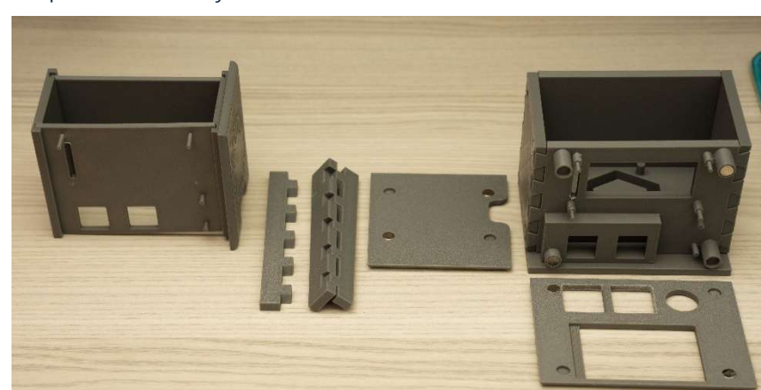
Version 1 pictured on the left, Dovetail joint tests in the middle, and Version 2 pictured on the right
