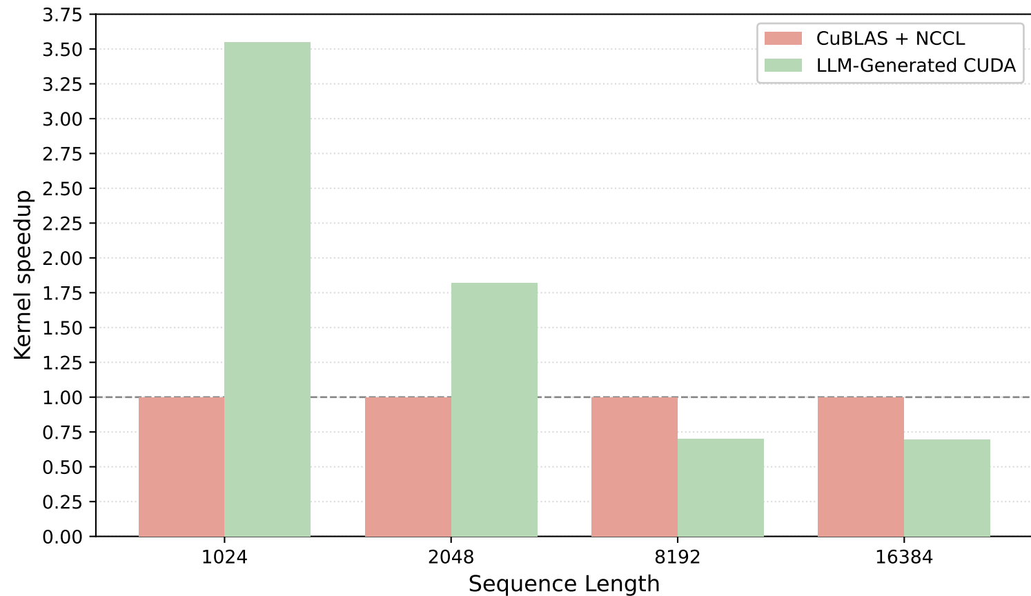
Hyena CP Speedup: Reference vs. GPT-5.5-generated Kernel
