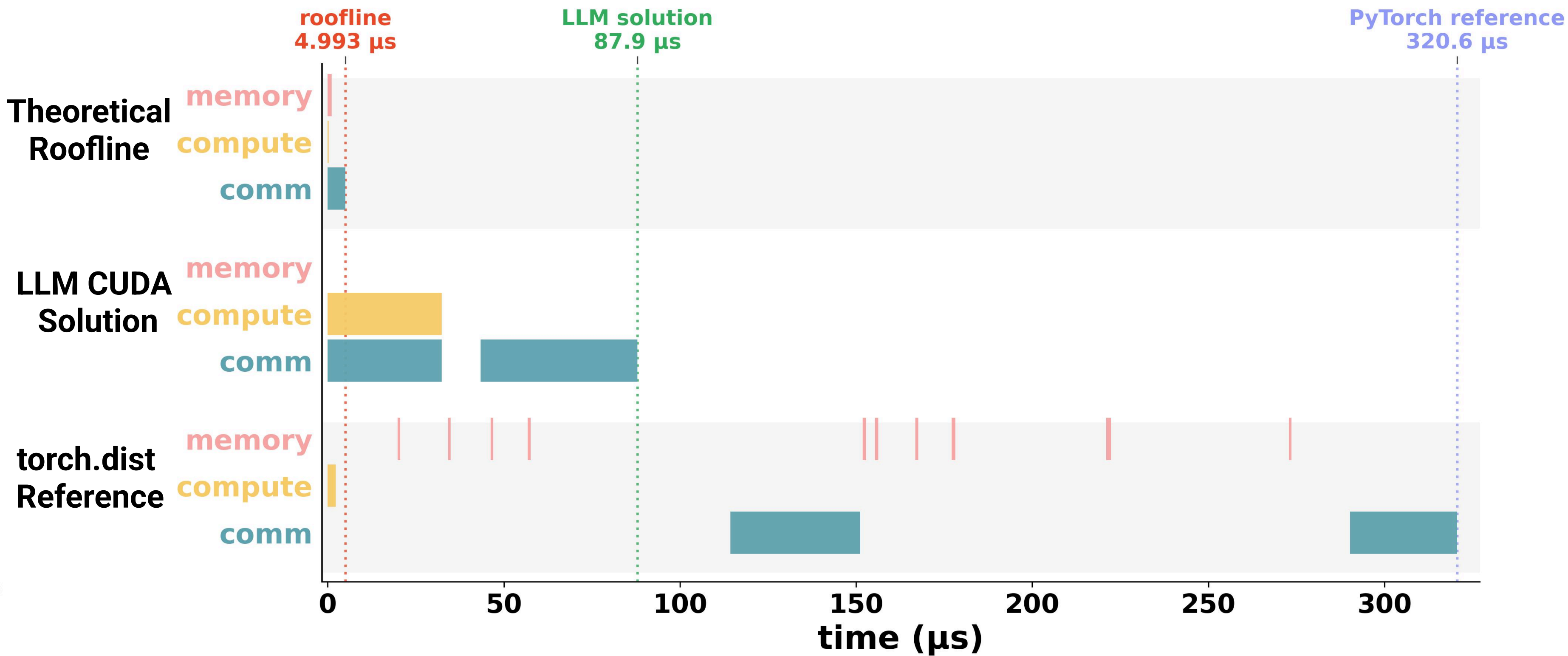
GEMM + All-Gather: Roofline vs PyTorch vs LLM CUDA Solution
