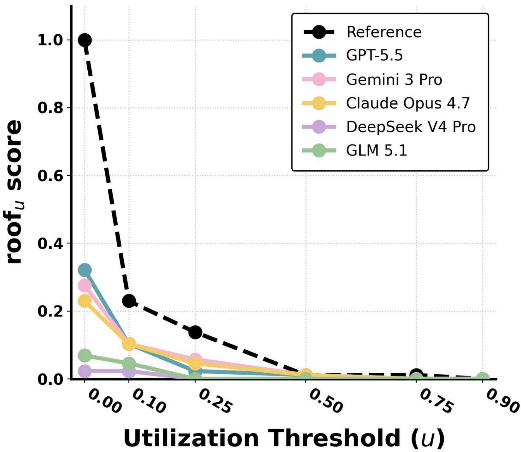
\text{roof}_u distribution of different models
