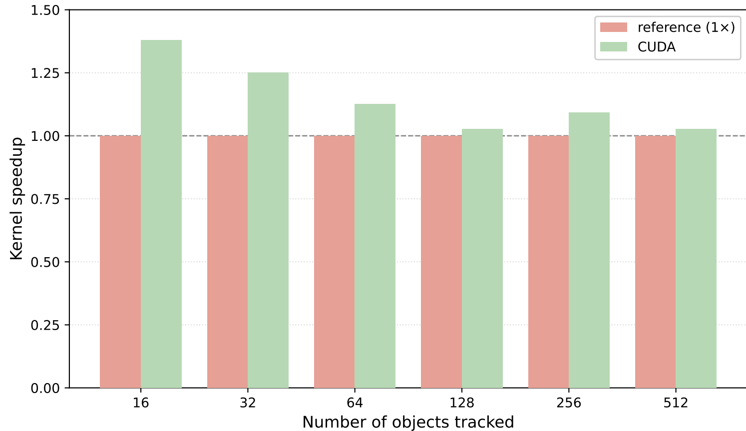
SAM3 IoU Suppression Speedup: Reference vs. GPT-5.5-generated Kernel
