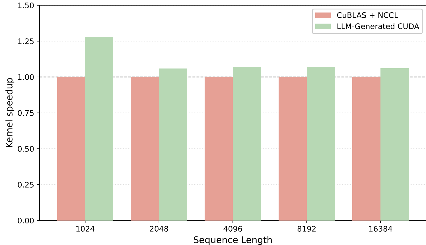
Vocab Parallel Log-Prob Top-K Speedup: Reference vs. Gemini 3 Pro-generated Kernel
