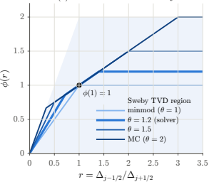
(a) Generalized-minmod family
