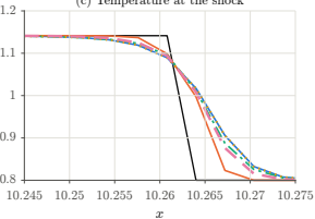
(c) Temperature at the shock
