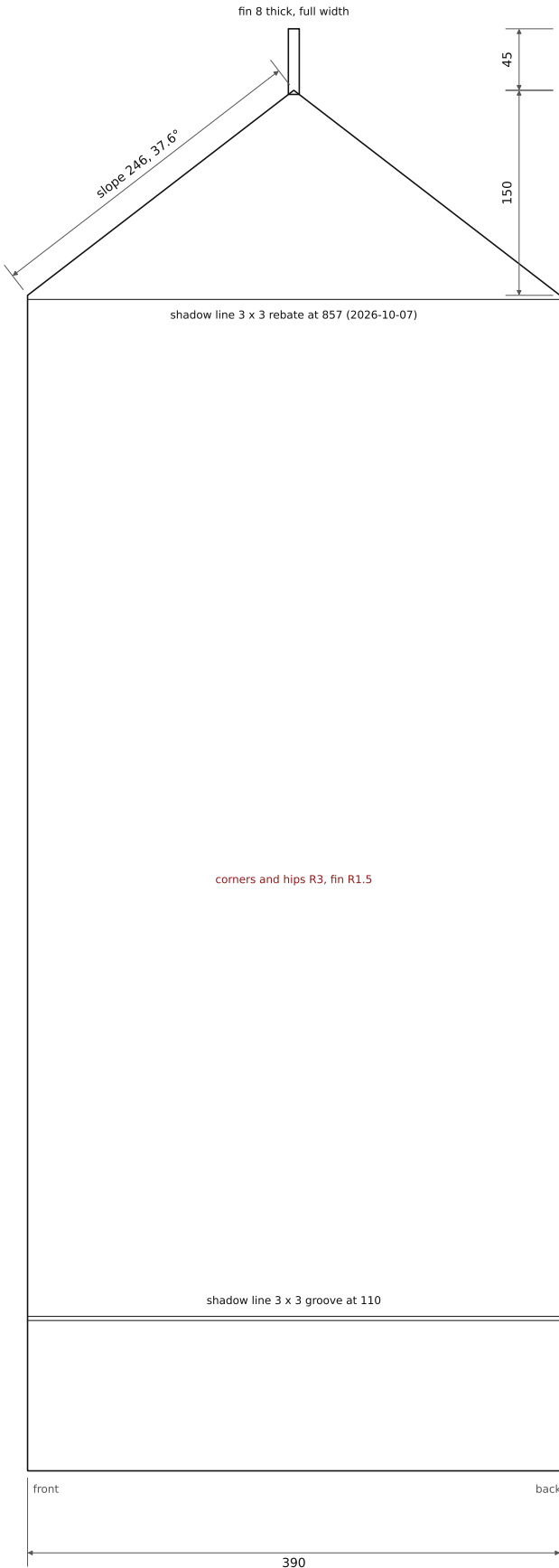
RIGHT SIDE
