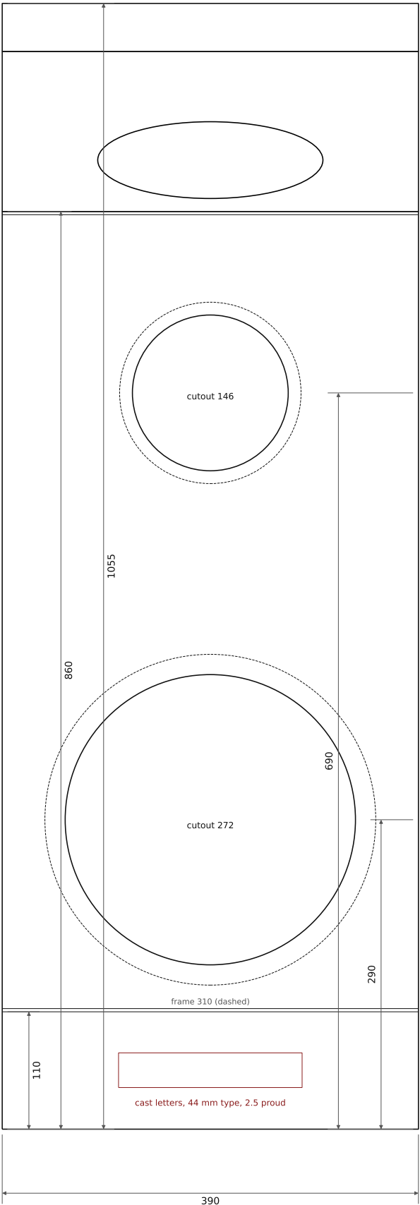
FRONT
