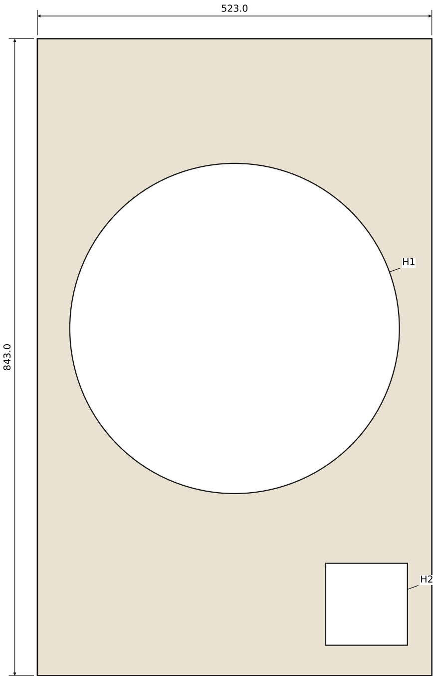
cork-face: 3 mm cork, 2 for the set, seen from its outer face (option: cork-face)
