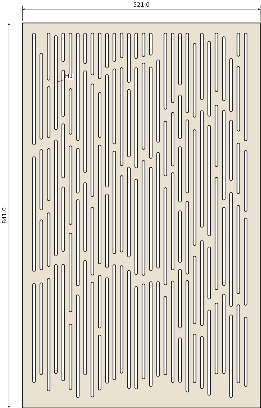
grille-strips: 6 mm spotted-gum-ply, 2 for the set, seen from its outer face (option: strip-grille)
