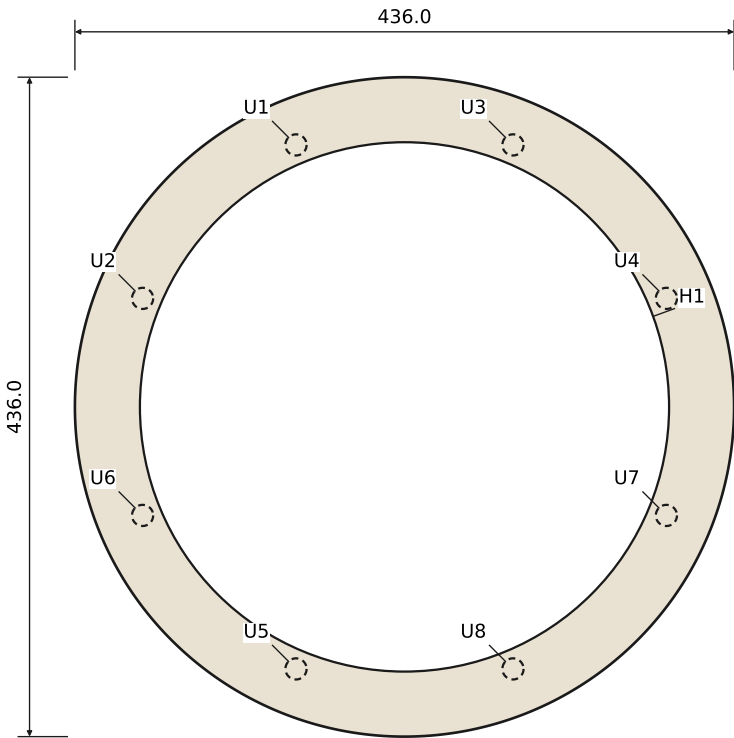
woofer-ring: 6 mm mdf, 2 for the set, seen from its outer face inner-face pockets: dxf/woofer-ring-underside.dxf (seen from that face)
