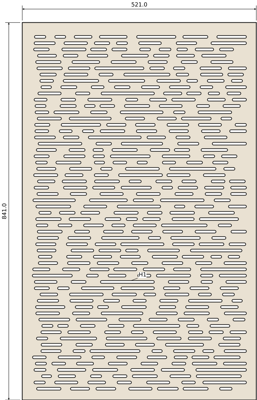
grille-lenticel: 6 mm baltic-birch, 2 for the set, seen from its outer face (option: lenticel-grille)
