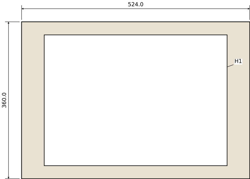
brace: 18 mm baltic-birch, 2 for the set, seen from its outer face
