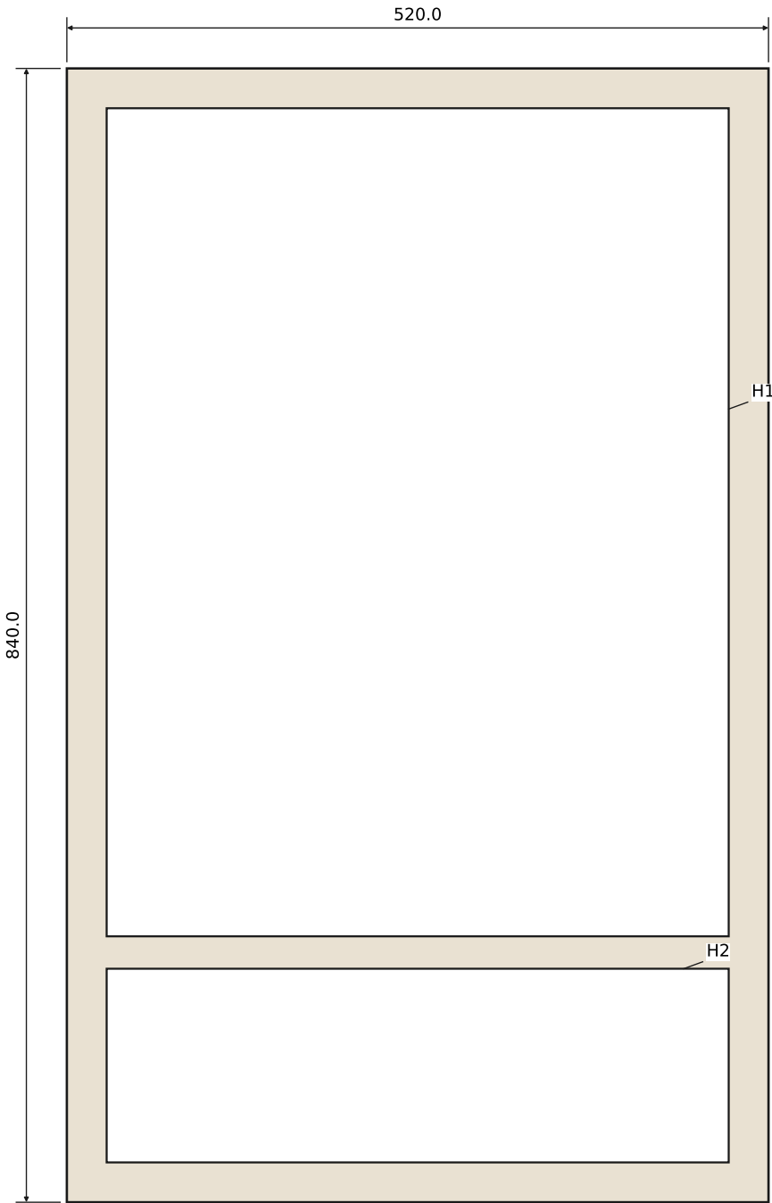
cloth-frame: 6 mm mdf, 2 for the set, seen from its outer face (option: cloth)
