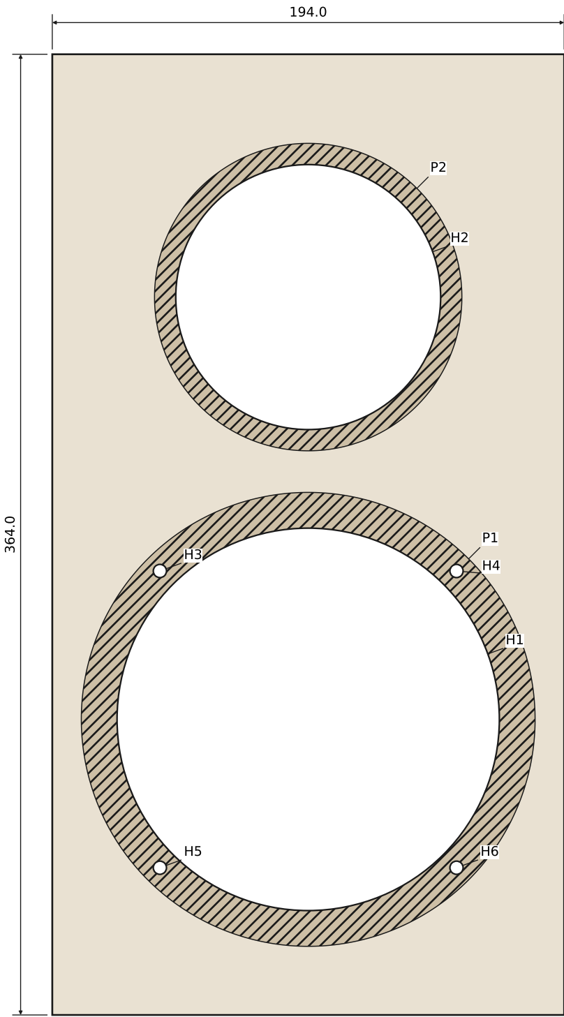
baffle: 18 mm baltic-birch, 2 for the set, seen from its outer face
