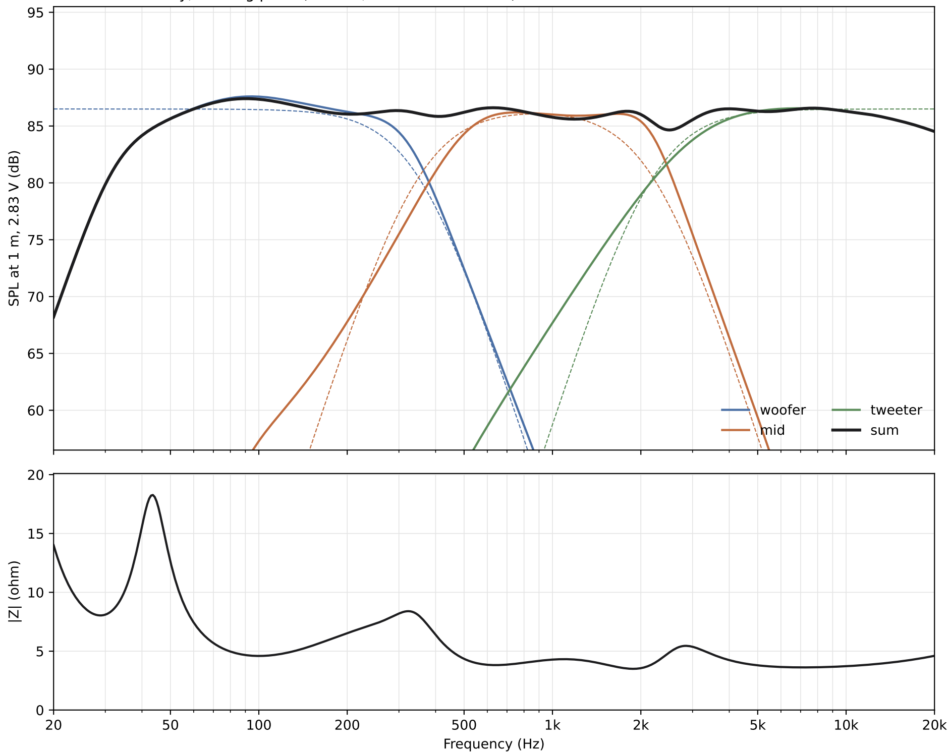
earnilk three-way, starting point (models, not measurements): LR4 at 350 Hz and 2200 Hz
