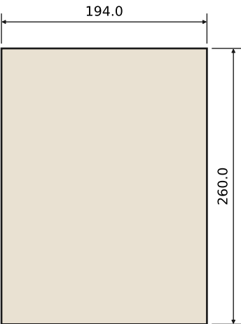
top, bottom 18 mm baltic-birch, 4 for the set
