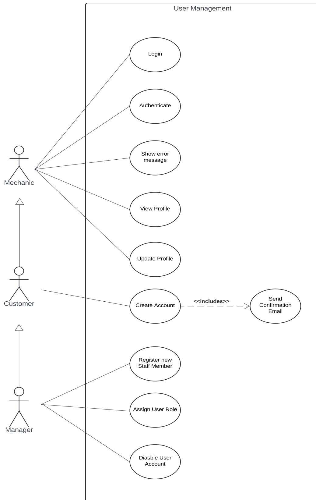
Figure 1: User Management Use Case Diagram
