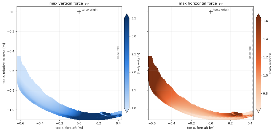
Figure 3.12: Static toe-force capability over the measured workspace: maximum vertical force F_z (left) and horizontal force F_x (right), in body weights, clipped at 3.5 BW. The vertical map feeds the flight-phase impulse bound.
