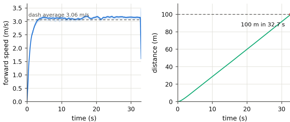
Figure 5.2: One of the greedy evaluation of the sprint policy: forward speed over the dash (left) and cumulative distance against the 100 m target (right).
