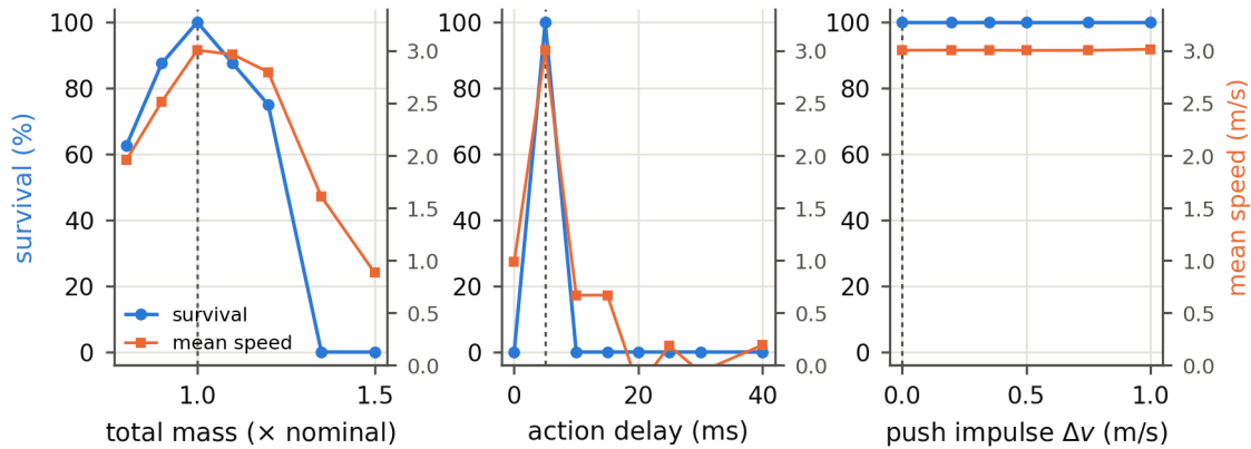
Figure 5.4: Robustness margins of the sprint policy under greedy evaluation: survival rate and mean speed against total mass scaling (left), action delay (centre), and push impulse (right). The dashed line marks the nominal training value.
