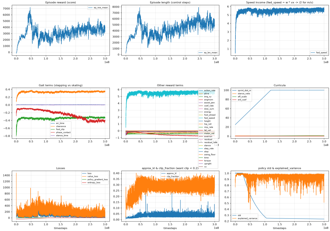
Figure 5.3: Training diagnostics for the sprint policy: episode reward and length, forward-speed reward income, gait and other reward terms, curriculum schedules, losses, PPO clip statistics, and policy standard deviation with explained variance, all against timesteps.
