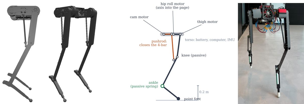
Figure 3.1: DASH-01, from the simulated model and in picture.
