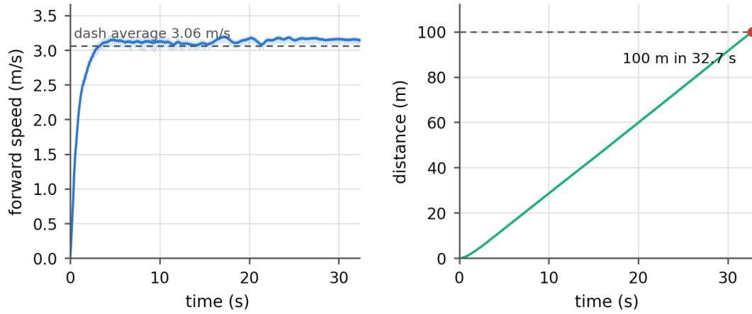
Figure 5.1: One of the greedy evaluation of the sprint policy: forward speed over the dash (left) and cumulative distance against the 100 m target (right).
