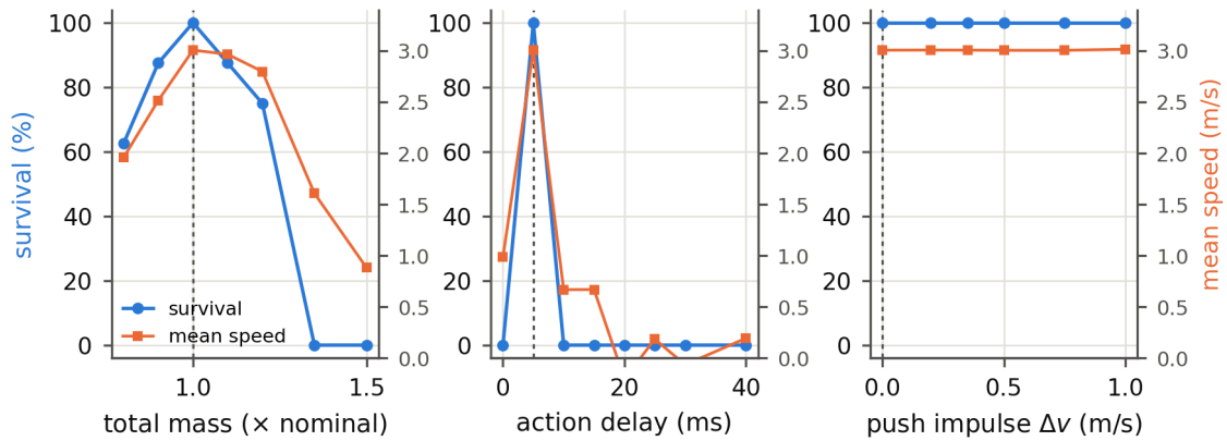
Figure 5.5: Robustness margins of the sprint policy under greedy evaluation: survival rate and mean speed against total mass scaling (left), action delay (centre), and push impulse along the fore-aft axis (right). The dashed line marks the nominal training value.
