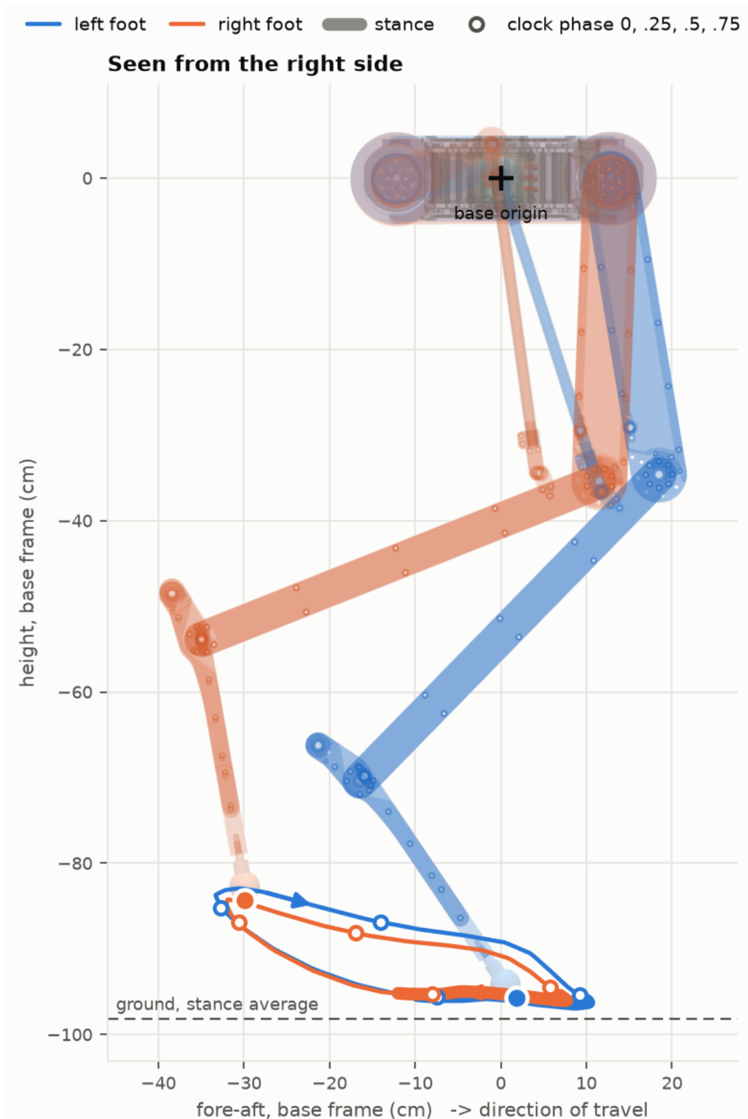
Figure 5.4: Gait in end effector space
