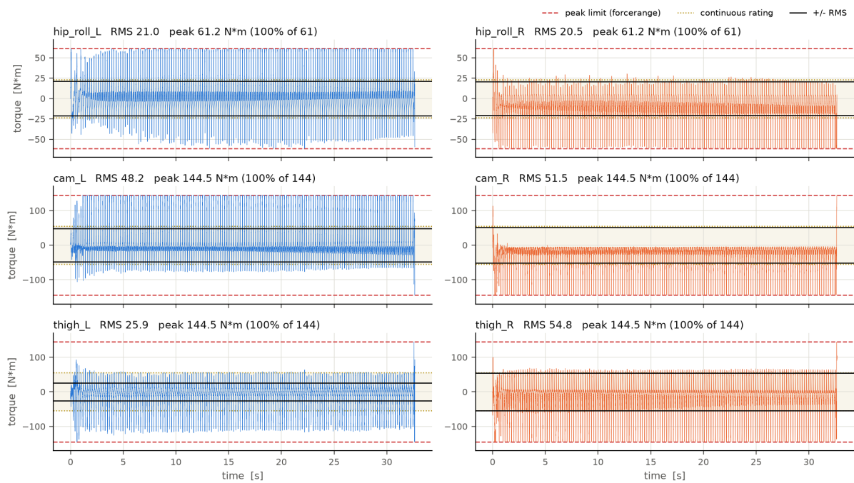
Figure 5.3: Torque of the actuator during the 100m dash
