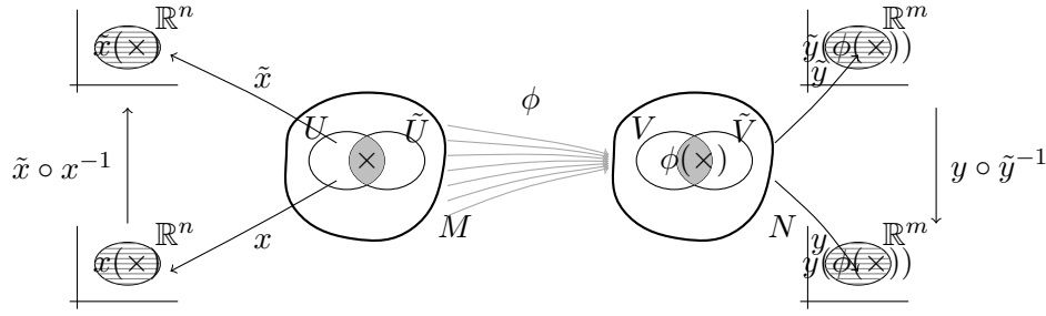
Fig: Amateur's depiction of a diffeomorphism \phi
