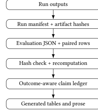
Figure 2: Evidence admission and interpretation. Invalid or irreproducible bundles stop at the gate; valid negative outcomes enter the ledger without supporting positive claims.
