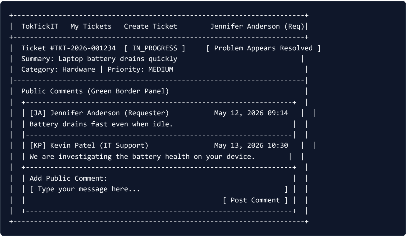
Real Implemented Requester Ticket View Screenshot
