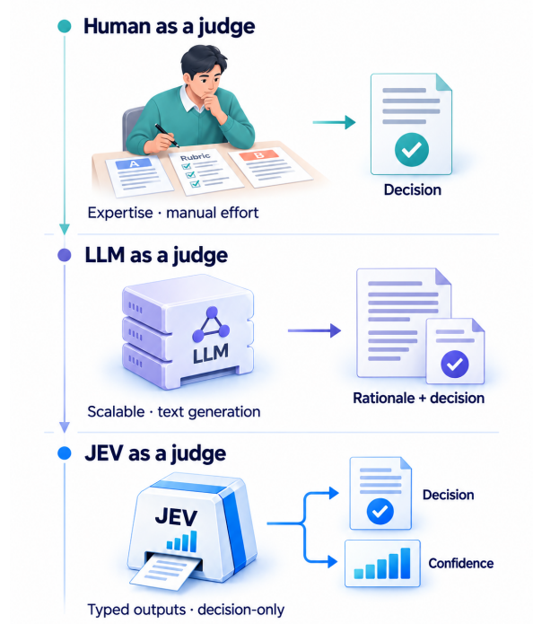
Figure 1: From human assessment to decision-only judging. Human evaluation relies on manual expertise, and generative LLM judges can produce a rationale alongside a decision; JEV exposes a typed decision and label probabilities, summarized as confidence. The diagram contrasts interfaces only: in our experiments, generative judges also answer under JEV’s decision-and-probability contract, without a rationale.
