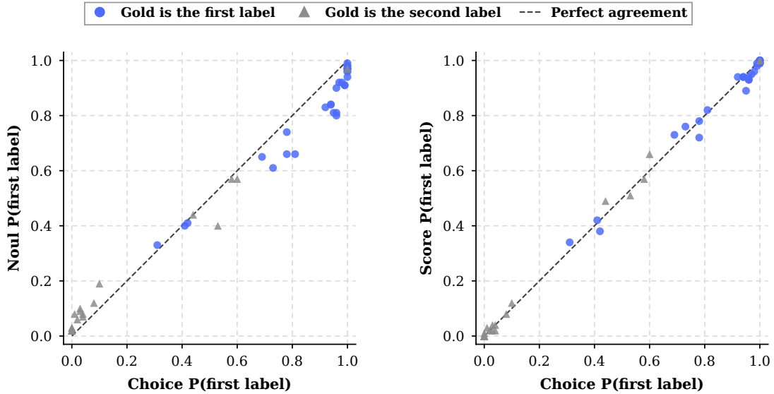
Figure 18: Initial-round primitive audit on 48 examples, with probabilities aligned to the same semantic label; color and marker show which label is gold. Co-question context and stochastic effects accompany differences among primitives.
