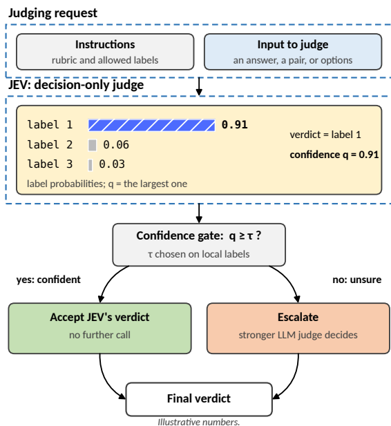
Figure 2: Accept when confident, escalate when unsure. JEV returns a decision and label probabilities; their maximum is the confidence signal. Confident decisions are accepted, and uncertain inputs are escalated to a stronger LLM judge whose decision becomes the final verdict. The threshold is chosen and validated on the target workload. When the same request can be presented in several orders, the aligned probabilities can be averaged across presentations before gating; our pairwise cascades average both candidate orders.
