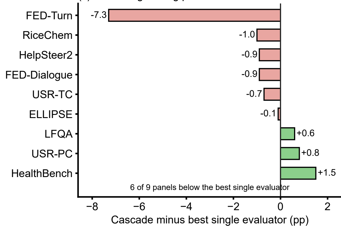
(c) Escalating among peer evaluators
