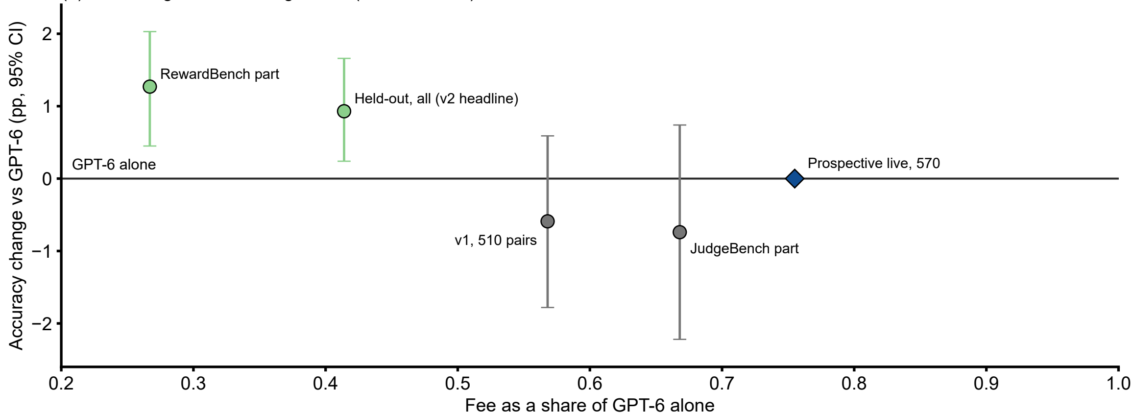
(a) Escalating to a reasoning model (Jev → GPT-6)
