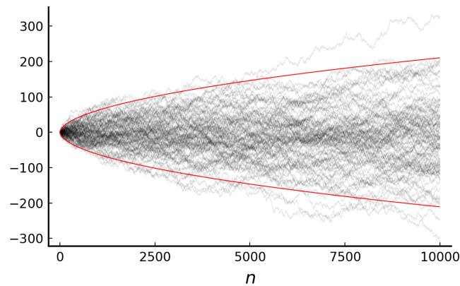
Black: 100 trials of (S_n) . Red: \pm\sqrt{2n \log \log n} .
