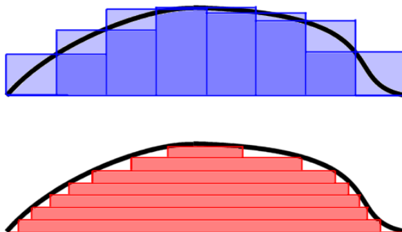
(Blue) Riemann integral. (Red) Lebesgue integral. ( source )
