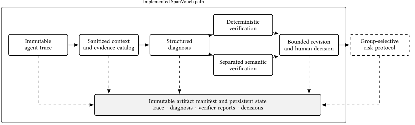
Figure 1: IVAD information and decision flow in SpanVouch. Solid boxes are implemented components exercised by the engineering validation. The dashed box is the formal group-selective protocol; the Technical Report specifies its conditional guarantee but does not report empirical target-risk attainment.
