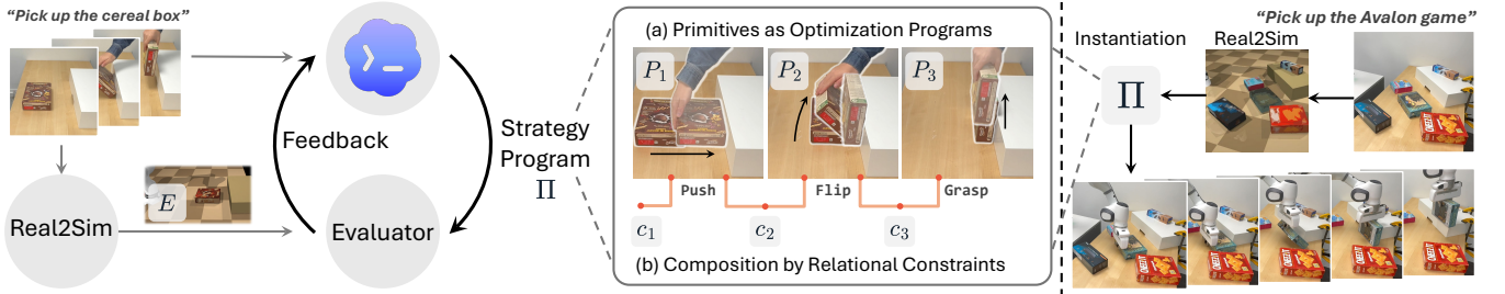
Closing the Agentic Loop from Demonstration Object-Centric Relational Program Representation Strategy Instantiation in Novel Scenes Fig. 2: Overview of RAPID. E is a simulation environment reconstructed from the demonstration, P_i 's are manipulation primitives, and \Pi is the strategy program generated by the coding agent.
