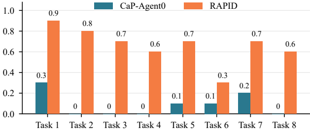
Success Rate
