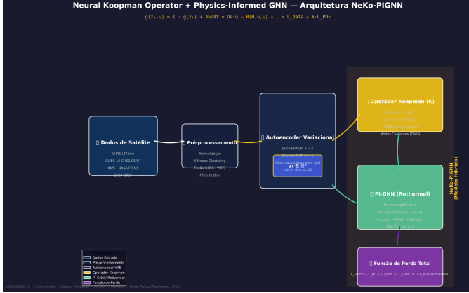
Figura 5: Neural Koopman Operator and PI-GNN hybrid architecture. Satellite data is encoded via VAE into Koopman observables, linearly propagated through matrix K , and spatially regularized by PI-GNN with Rothermel physical loss.
