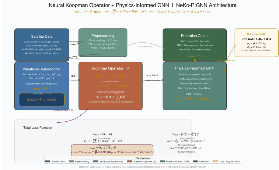
Figure 3: Hybrid Neural Koopman Operator and PI-GNN architecture. Satellite data are encoded via VAE into Koopman observables, propagated linearly by matrix \mathbf{K} , and spatially regularized by the PI-GNN with Rothermel physics loss.
