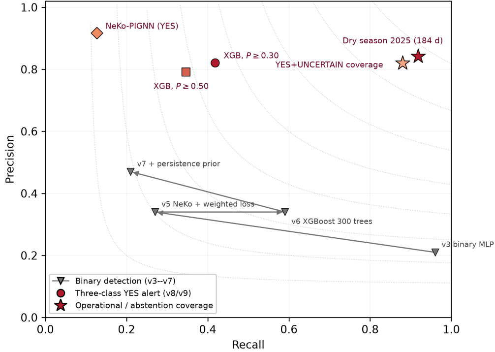
Figure 9: Published Exp-B operating points in precision–recall space (dotted lines: iso-F1 contours). Gray arrows trace the binary-detection iteration (v3→v7, Table 13); red markers show three-class YES alerts on the 20-day holdout (Table 12); stars show combined YES+UNCERTAIN coverage (Table 12) and the dry-season 2025 operational point (184 days, Table 15).
