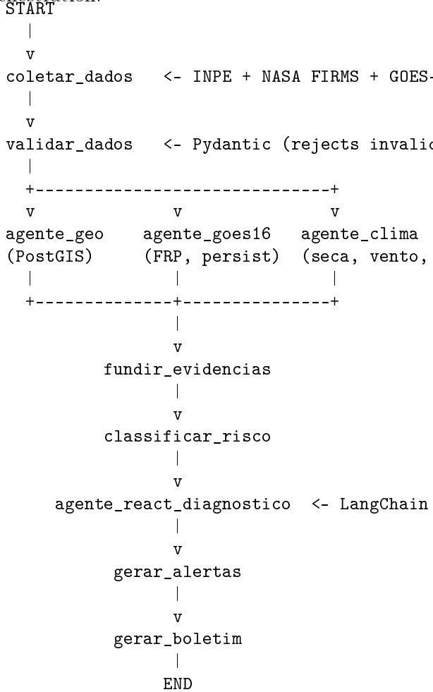
Figure 1: LangGraph pipeline for fire digital twin orchestration.
