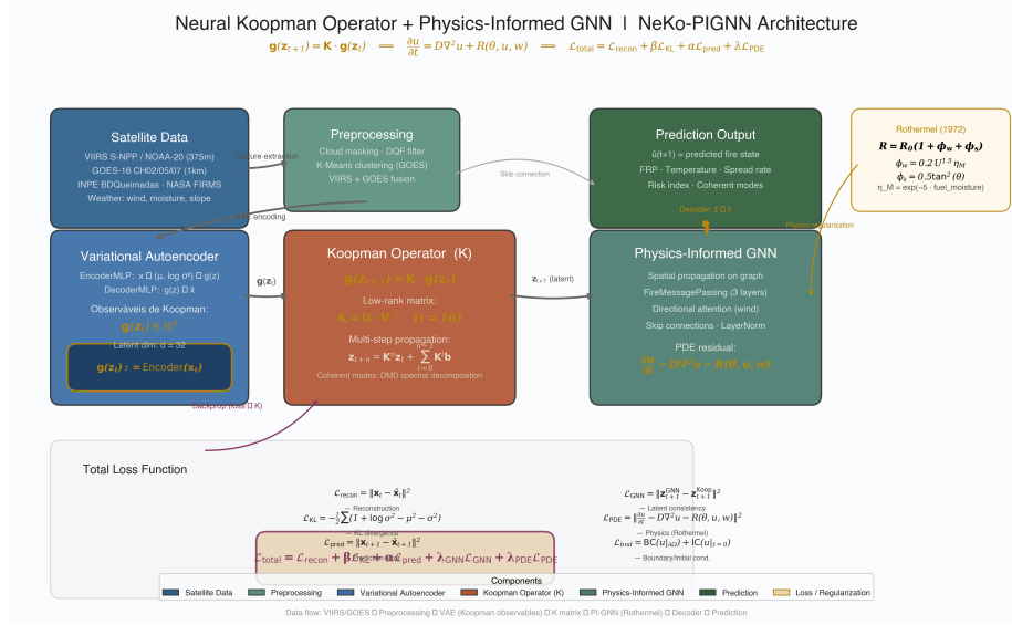
Figure 6: Hybrid Neural Koopman Operator and PI-GNN architecture. Satellite data are encoded via VAE into Koopman observables, propagated linearly by matrix \mathbf{K} , and spatially regularized by the PI-GNN with Rothenmel physics loss.
