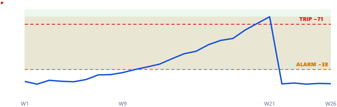
FIG. 5 - KO-3201 DE VIBRATION, 26 WEEKS (MICRON) - LIVE TRACE
