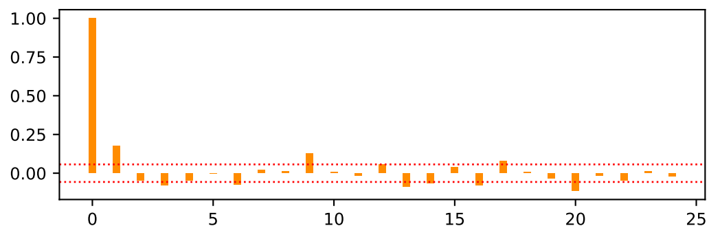
PACF of BIG.LoBM
