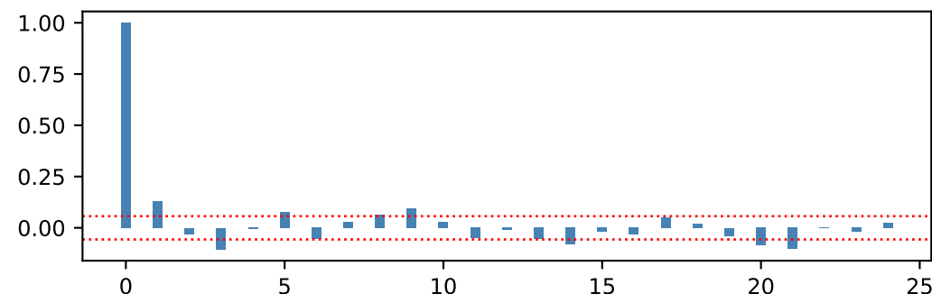
ACF of BIG.HiBM
