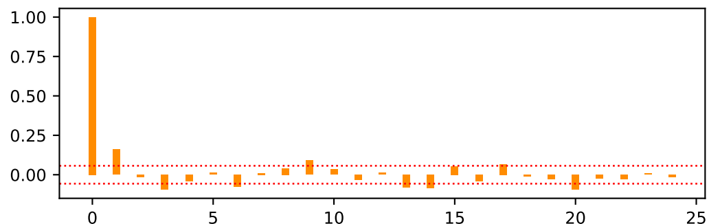
PACF of SMALL.HiBM
