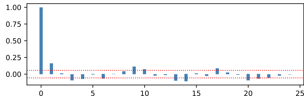
ACF of SMALL.HiBM
