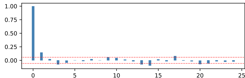
ACF of ME1.BM2
