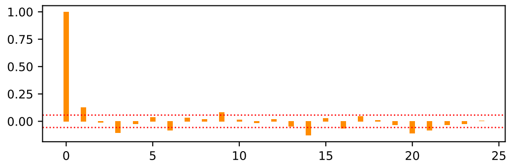
PACF of BIG.HiBM
