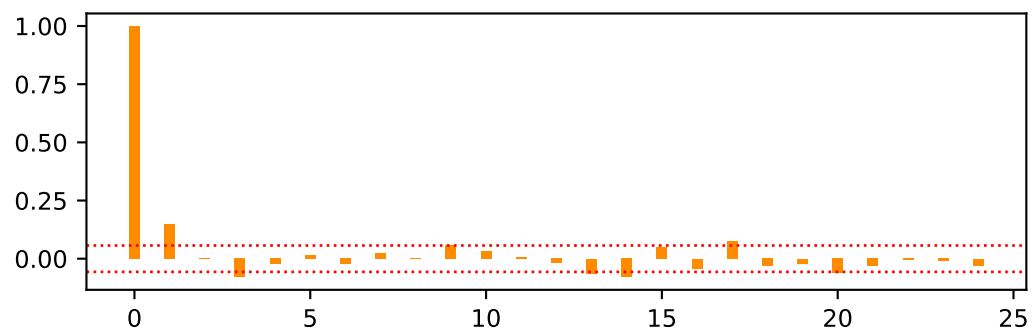
PACF of ME1.BM2
