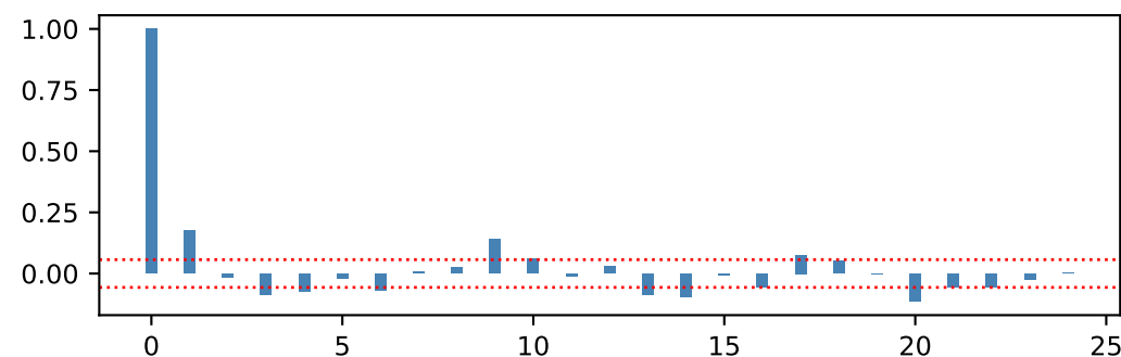
ACF of BIG.LoBM
