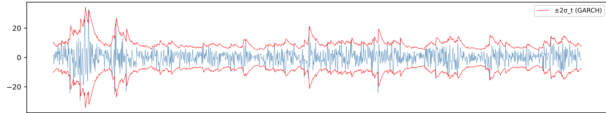
Estimated conditional standard deviation \sigma_t
