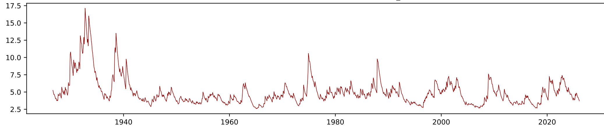
Estimated conditional standard deviation \sigma_t
