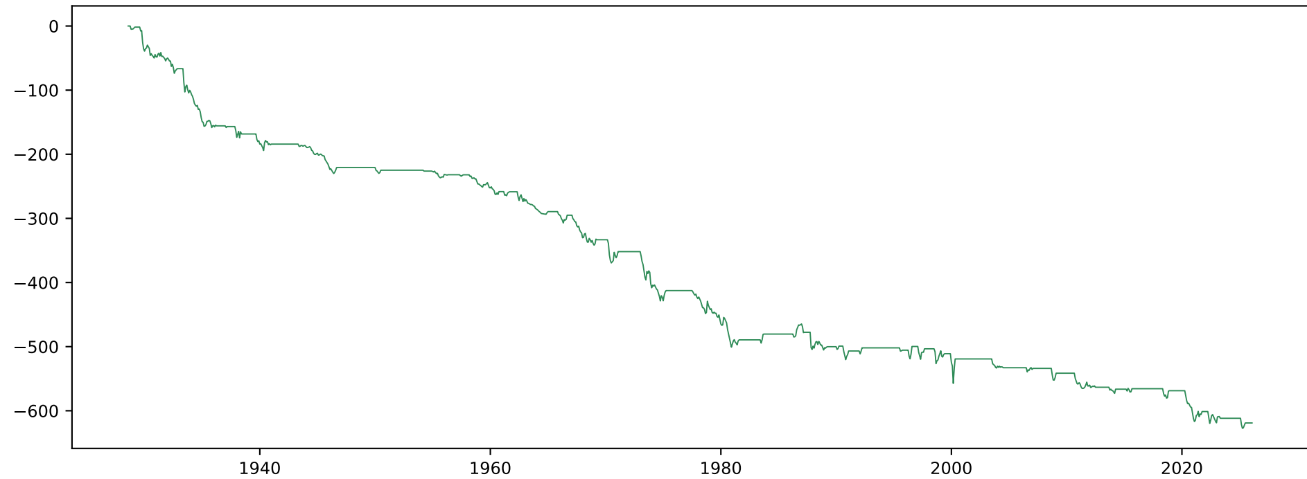
Cumulative P&L of the pairs trading strategy
