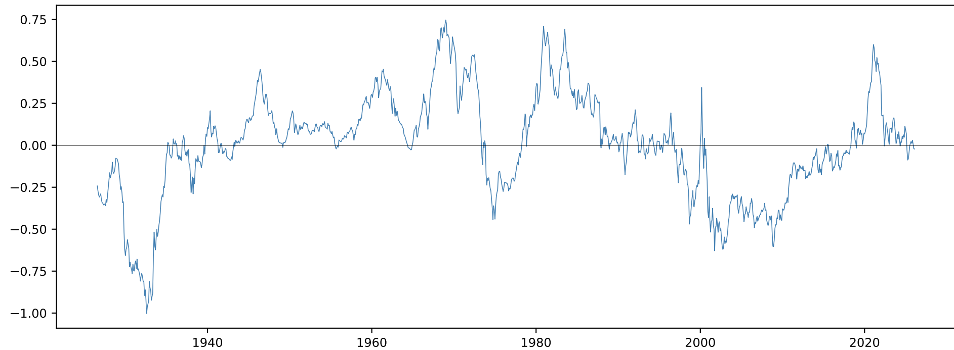
Cointegration spread: \text{SMALL.LoBM} - 0.70 \cdot \text{BIG.HiBM}
