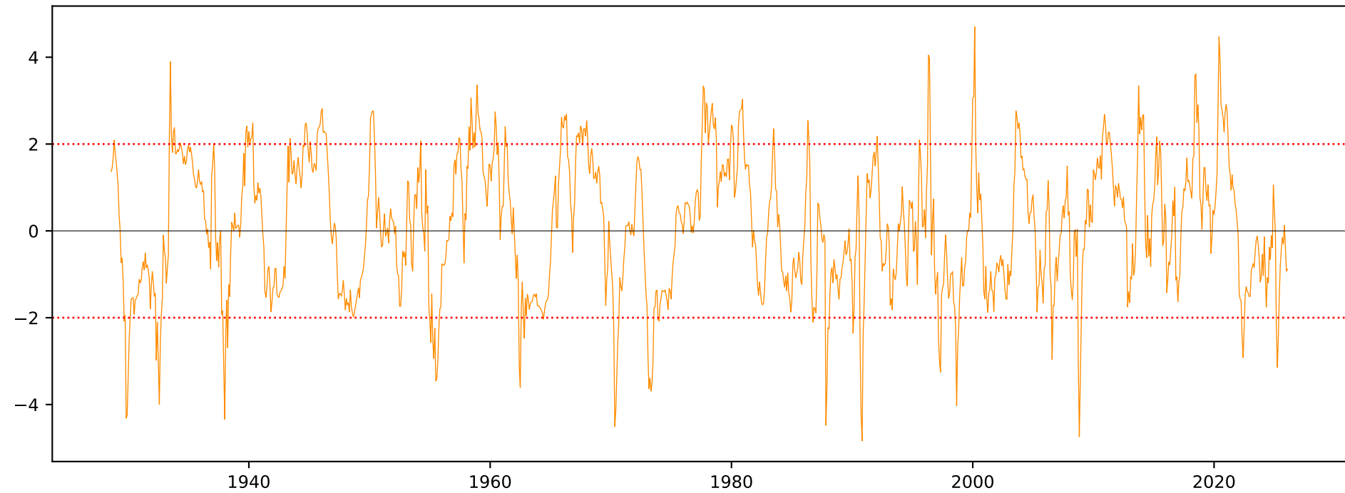
24-month rolling z-score of the spread
