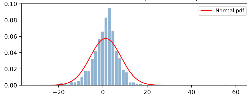
BIG.LoBM (skew=-0.13, ex.kurt=5.20)
