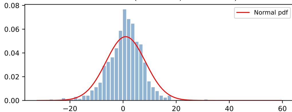
SMALL.HiBM (skew=1.96, ex.kurt=20.85)
