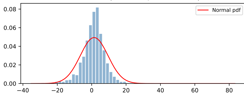
ME2.BM2 (skew=1.16, ex.kurt=17.20)
