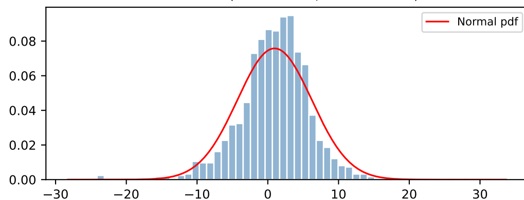
BIG.HiBM (skew=1.44, ex.kurt=17.45)
