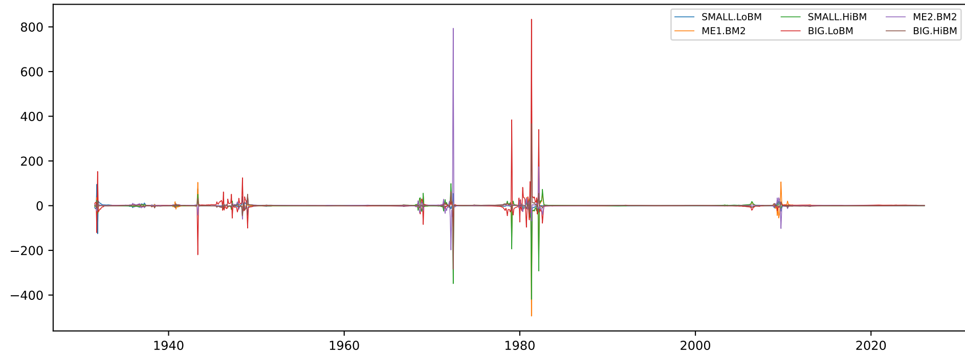
Shrinkage tangency weights through time
