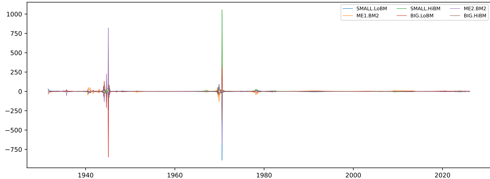
Plug-in tangency weights through time
